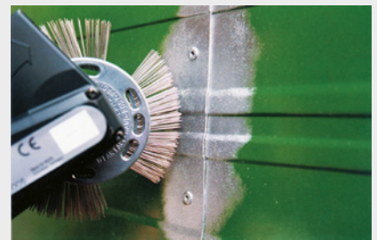
Removal of paint and corrosion from aluminium vehicle bodywork and assemblies, especially for rivets on truck bodies. No sand blasting effect!
